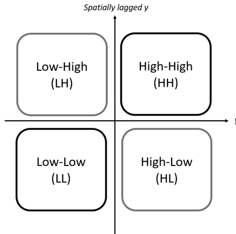
Figure II.3. Moran’s scatterplot
